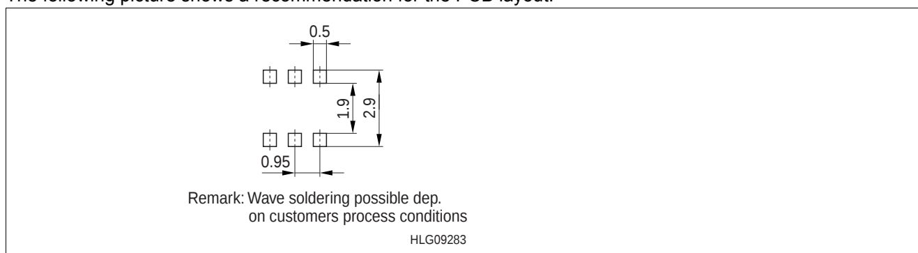
Figure 10 Footprint PG-TSOP-6-6-5
