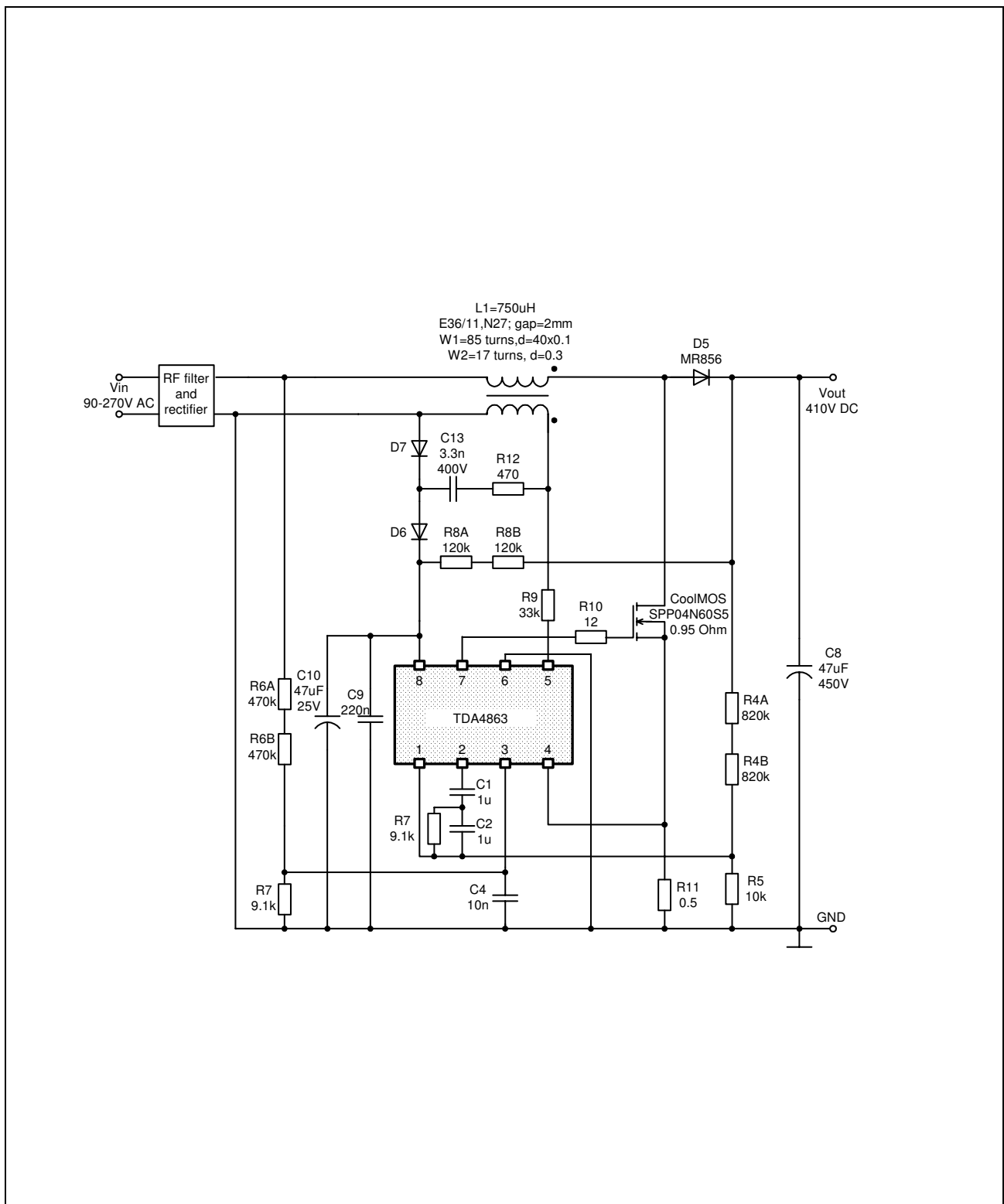
Figure 5 P_{\text{out}} = 110 \text{ W} , Universal Input V_{\text{in}} = 90 - 270 \text{ V AC}
