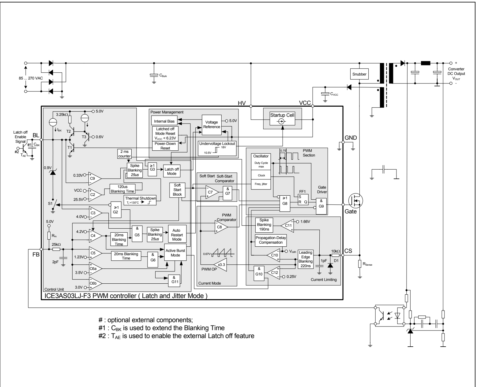
Figure 2 Representative Blockdiagram
