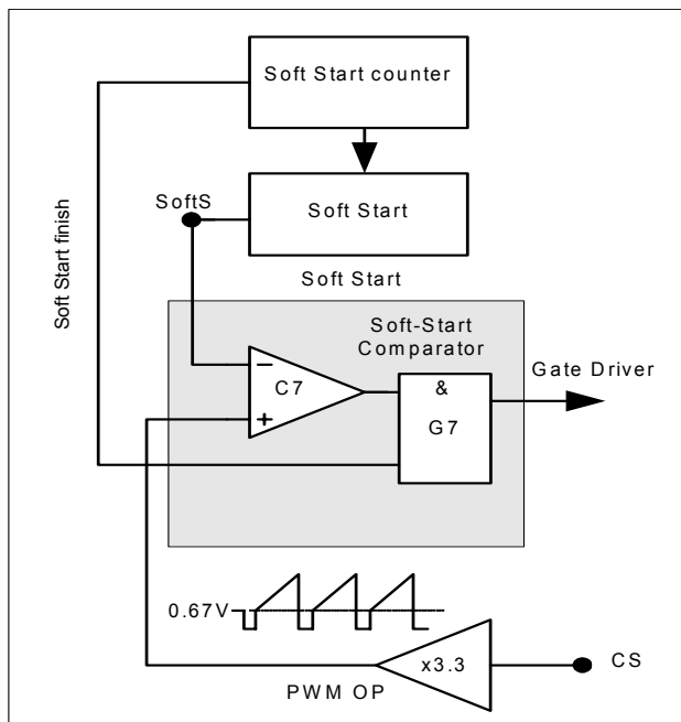
Figure 9 Soft Start
