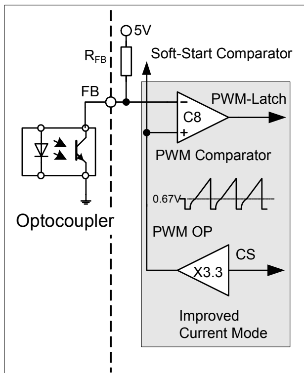
Figure 8 PWM Controlling
