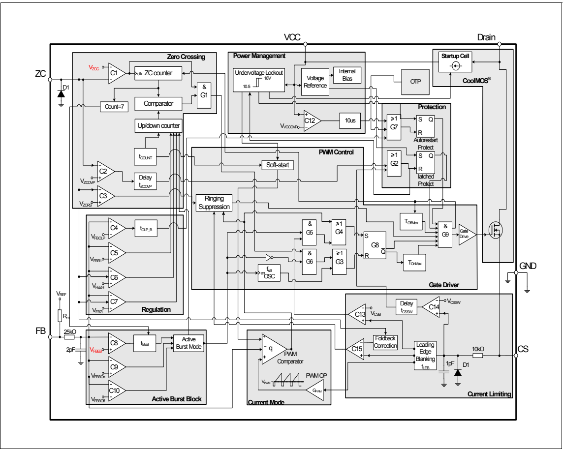
Figure 2 Representative Block diagram
