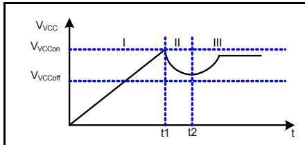
Figure 3 VCC voltage at start up
