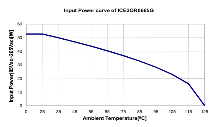
Figure 12 Input Power curve V_{in}=85\sim 265\text{Vac} ; P_{in}=f(T_a)
