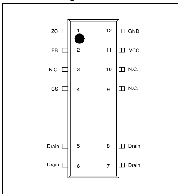
Figure 1 Pin Configuration PG-DSO-16/12 (top view)
