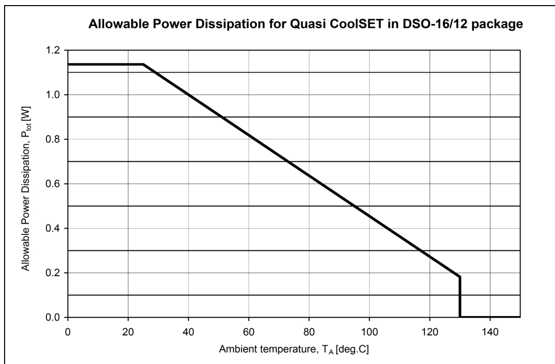
Figure 10 Power dissipation; P_{tot}=f(T_a)
