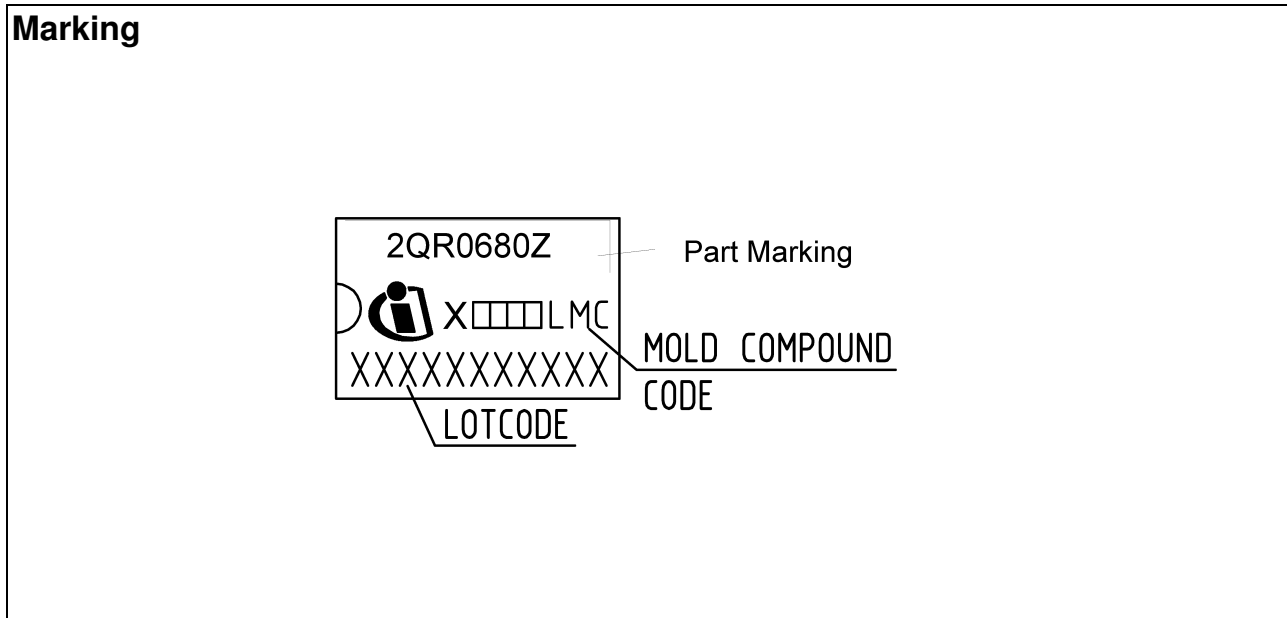
Figure 14 Marking for ICE2QR0680Z
