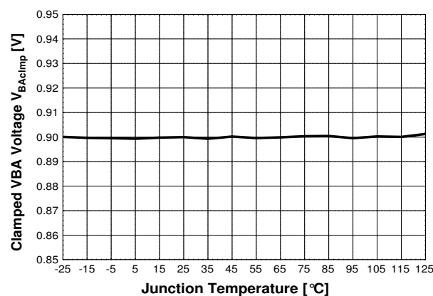
Figure 44 Clamped V_{BA} voltage V_{BAclmp}
