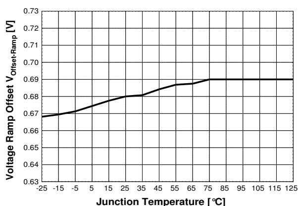
Figure 42 Voltage Ramp Offset V_{Offset-Ramp}
