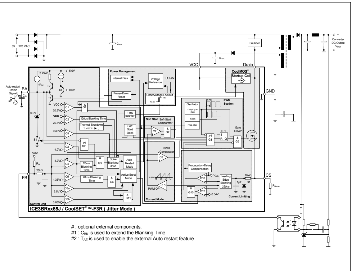
Figure 2 Representative Blockdiagram
