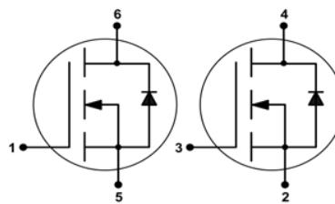
PG-TSOP6
