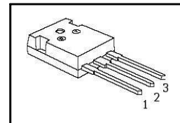
PG-TO247-3-1
