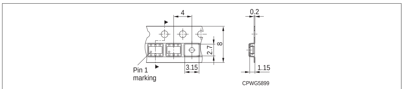
Figure 6 Tape loading
