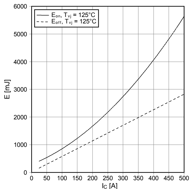
Schaltverluste IGBT-Wechselr. (typisch) switching losses IGBT-inverter (typical) E_{on} = f(I_C) , E_{off} = f(I_C) V_{GE} = \pm 15 \text{ V} , R_{Gon} = 3 \Omega , R_{Goff} = 20.4 \Omega , V_{CE} = 3600 \text{ V}
