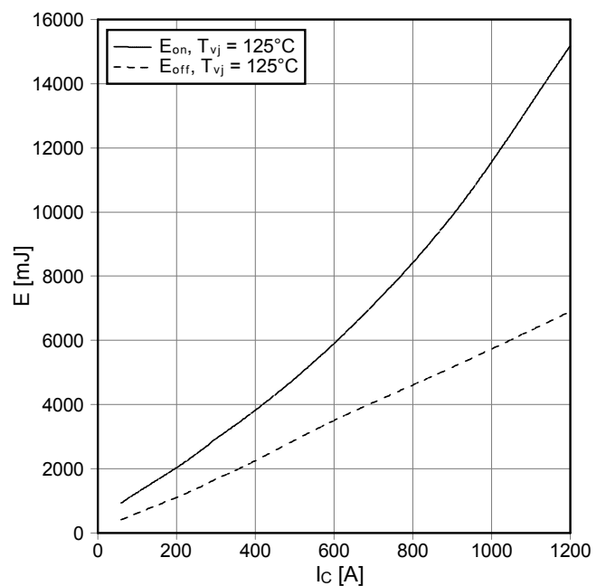
Schaltverluste IGBT-Wechselr. (typisch) switching losses IGBT-inverter (typical) E_{on} = f(I_C) , E_{off} = f(I_C) V_{GE} = \pm 15 \text{ V} , R_{Gon} = 4.3 \Omega , R_{Goff} = 30 \Omega , V_{CE} = 3600 \text{ V} , C_{GE} = 68 \text{ nF}
