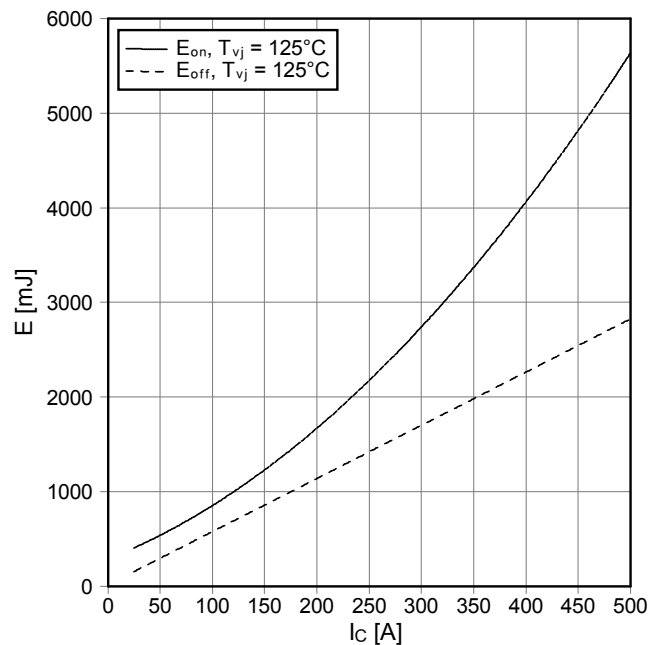
Schaltverluste IGBT-Wechselr. (typisch) switching losses IGBT-inverter (typical) E_{on} = f(I_C) , E_{off} = f(I_C) V_{GE} = \pm 15 \text{ V} , R_{Gon} = 3 \Omega , R_{Goff} = 20.4 \Omega , V_{CE} = 3600 \text{ V}
