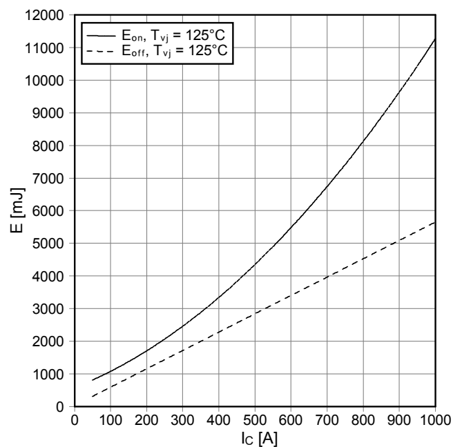
Schaltverluste IGBT-Wechselr. (typisch) switching losses IGBT-inverter (typical) E_{on} = f(I_C) , E_{off} = f(I_C) V_{GE} = \pm 15 \text{ V} , R_{Gon} = 1.5 \Omega , R_{Goff} = 10 \Omega , V_{CE} = 3600 \text{ V}
