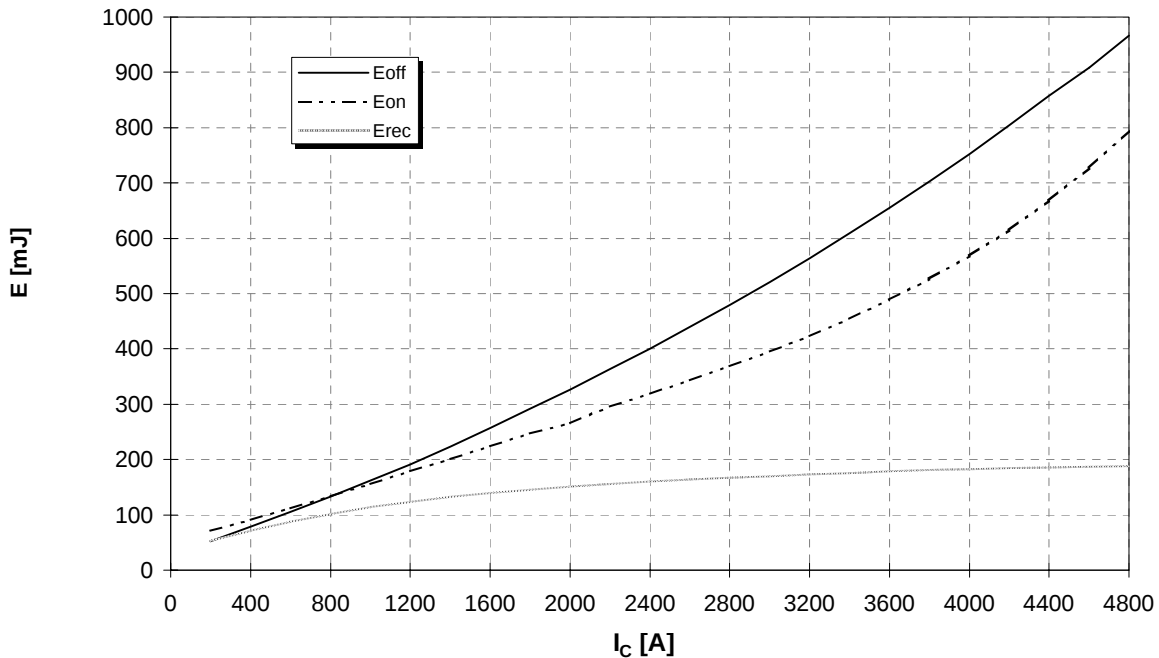
Schaltverluste (typisch) E_{on} = f(I_C) , E_{off} = f(I_C) , E_{rec} = f(I_C) Switching losses (typical) R_{gon} = R_{goff} = 0,56 \Omega , V_{CE} = 600V , T_J = 125^\circ C
