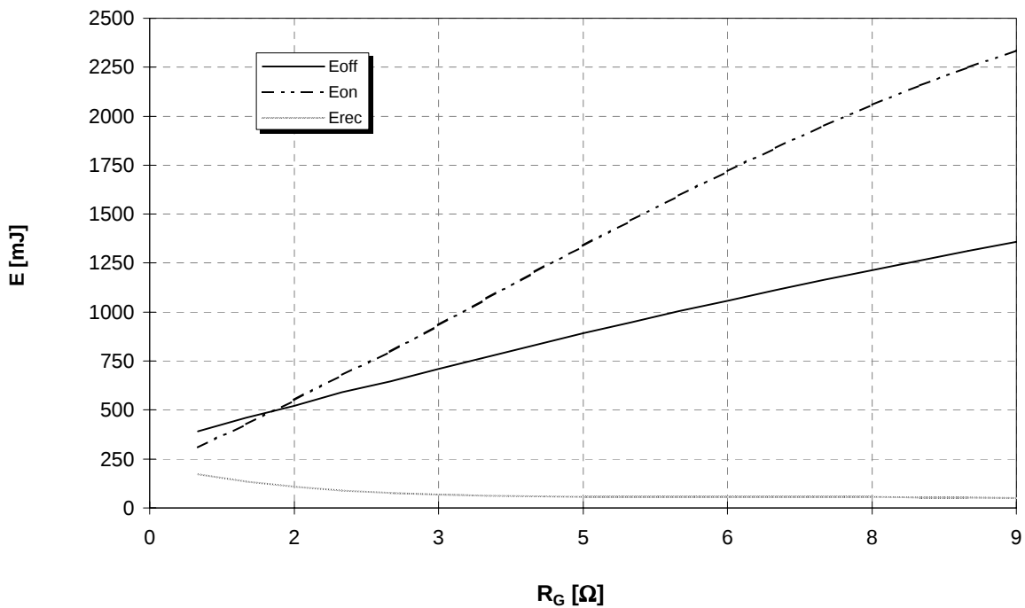
Schaltverluste (typisch) E_{on} = f(R_G) , E_{off} = f(R_G) , E_{rec} = f(R_G) Switching losses (typical) I_C = 2400A , V_{CE} = 600V , T_J = 125^\circ C
