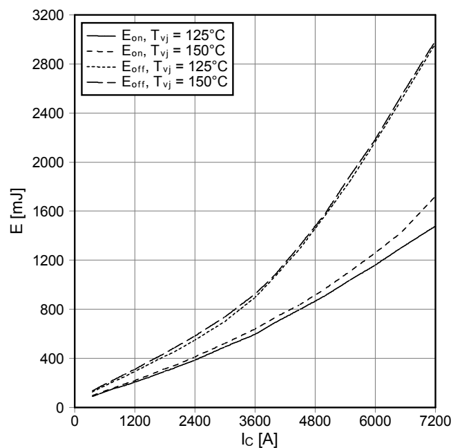
Schaltverluste IGBT-Wechselr. (typisch) switching losses IGBT-inverter (typical) E_{on} = f(I_C) , E_{off} = f(I_C) V_{GE} = \pm 15\text{ V} , R_{Gon} = 1.3\ \Omega , R_{Goff} = 0.22\ \Omega , V_{CE} = 600\text{ V}
