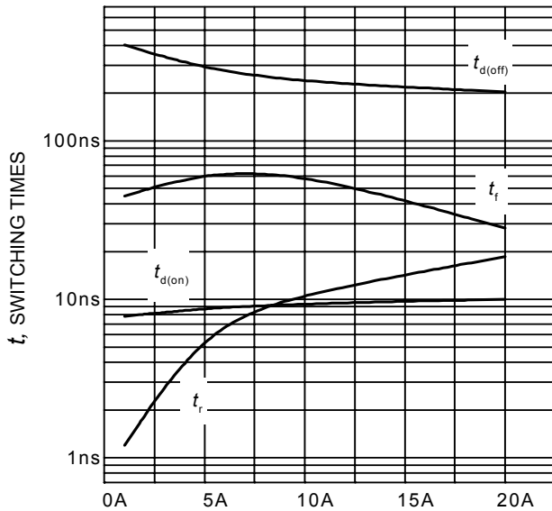
Figure 9. Typical switching times as a function of collector current (inductive load, T_J = 175^\circ\text{C} , V_{CE} = 400\text{V} , V_{GE} = 0/15\text{V} , R_G = 23\Omega , Dynamic test circuit in Figure E)
