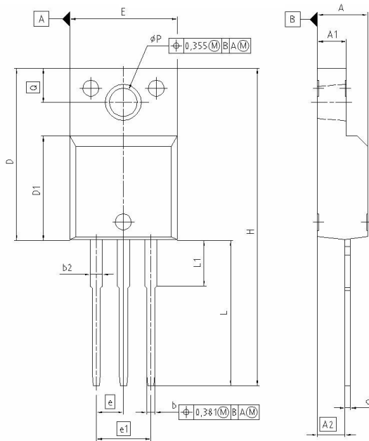
PG-TO220-3-31
