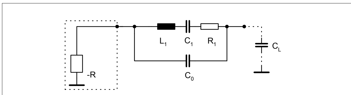
Figure 3-11 Crystal
