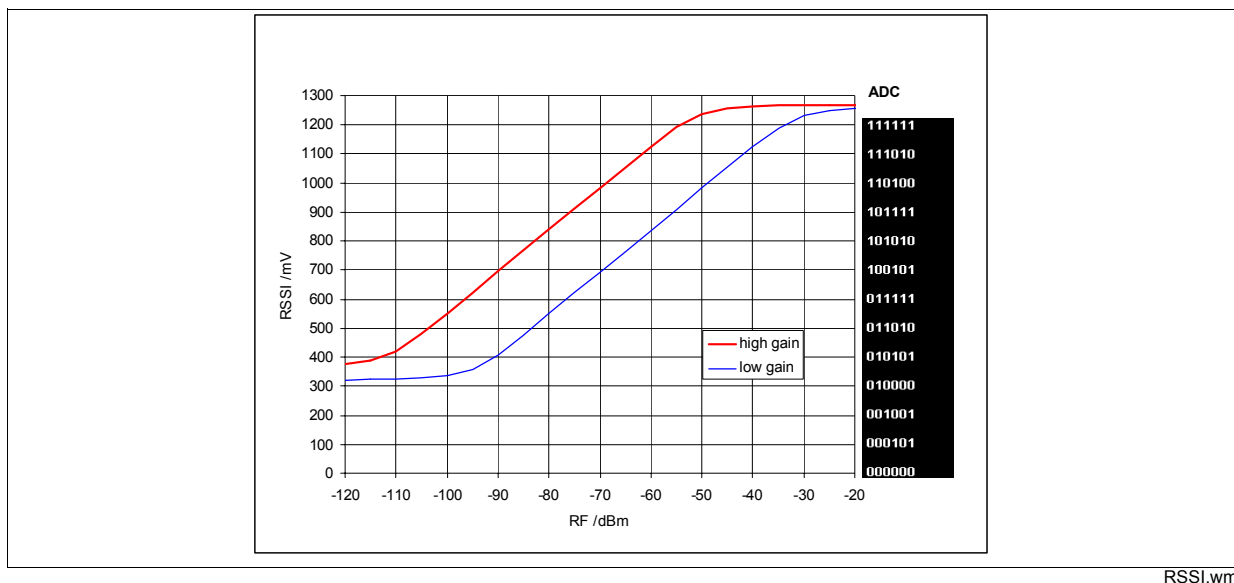
Figure 3-21 Typ. RSSI Level (Eval Board) @3V
