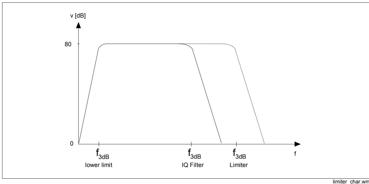
Figure 3-20 Limiter frequency characteristics
