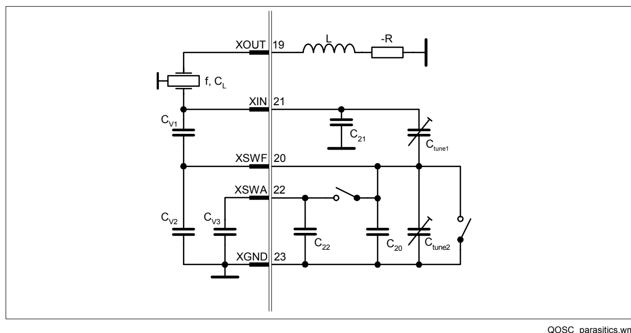
Figure 3-16 parasitics of the switching network
