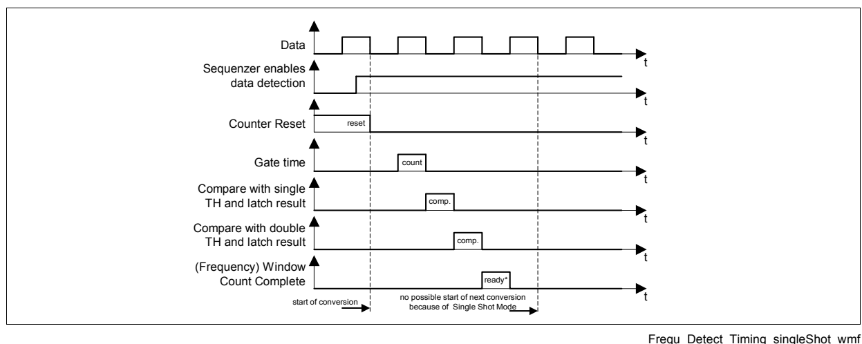
Figure 3-29 Frequency Detection timing in Single Shot mode
