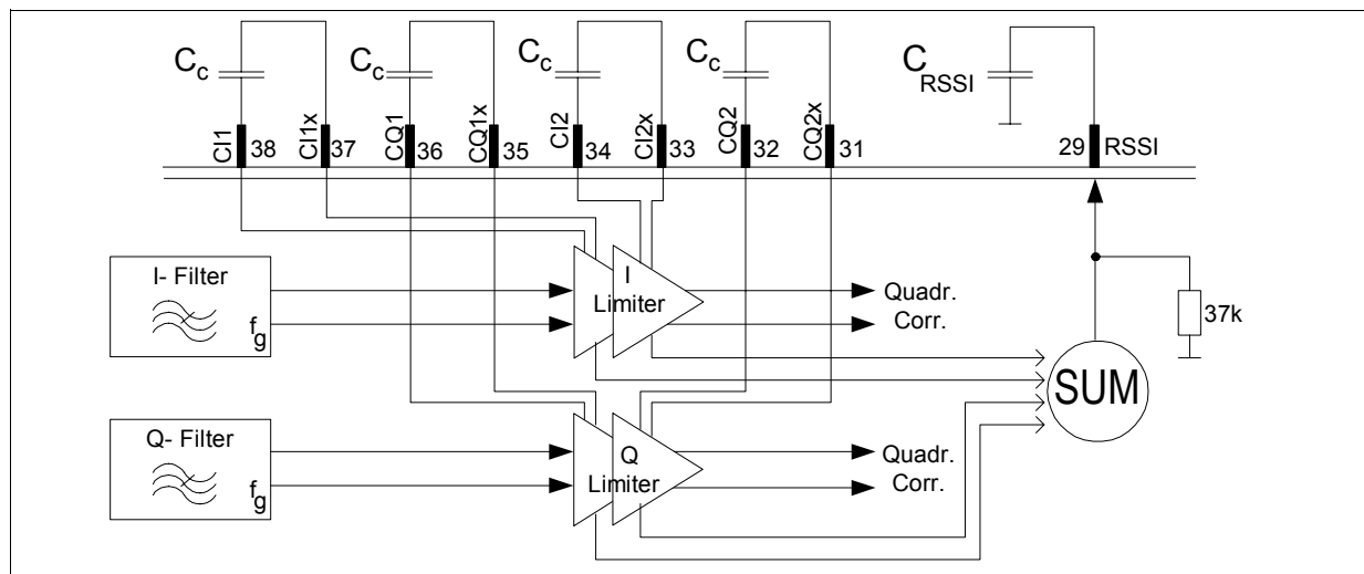
Figure 3-19 Limiter and Pinning
