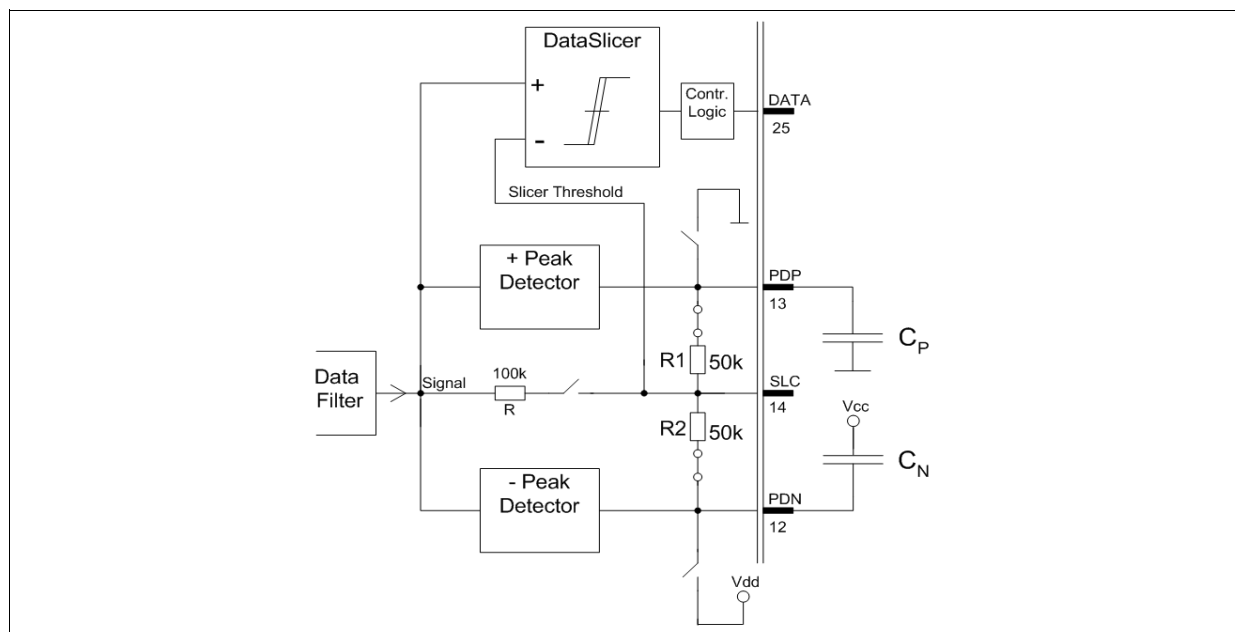
Figure 3-23 Slicer Level using Peak Detector
