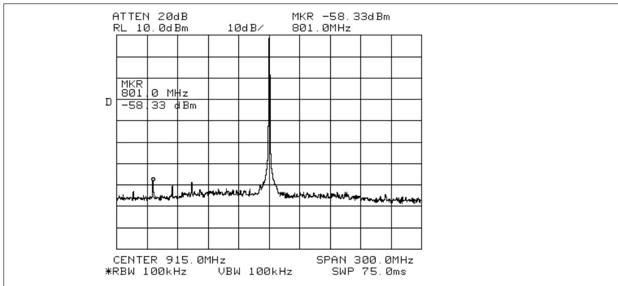
Figure 3-10 Transmit Spectrum 300MHz
