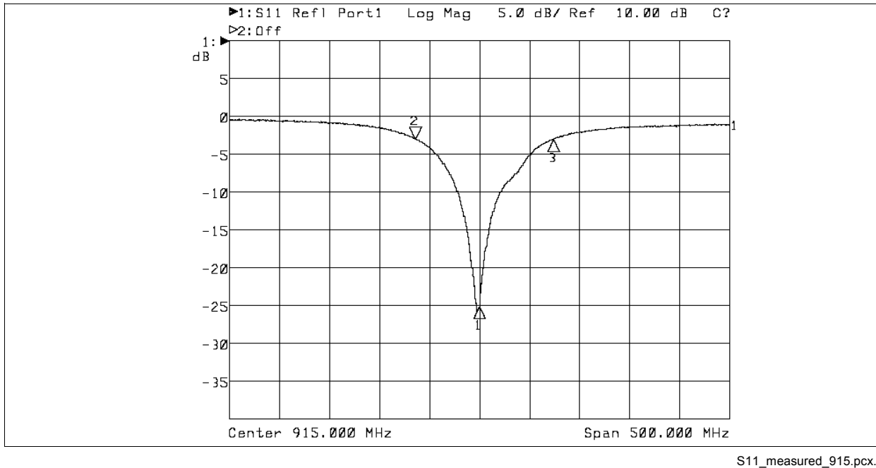
Figure 3-3 S11 measured
