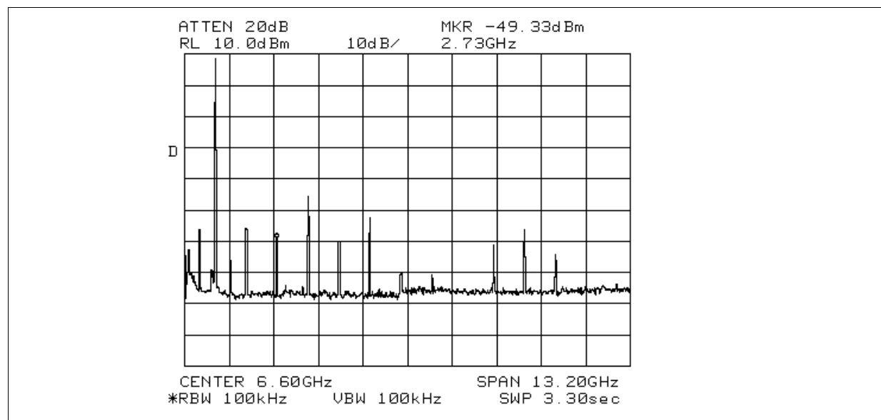
Figure 3-9 Transmit Spectrum 13.2GHz
