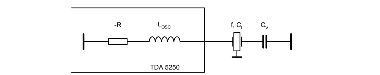
Figure 3-12 Crystal Oscillator
