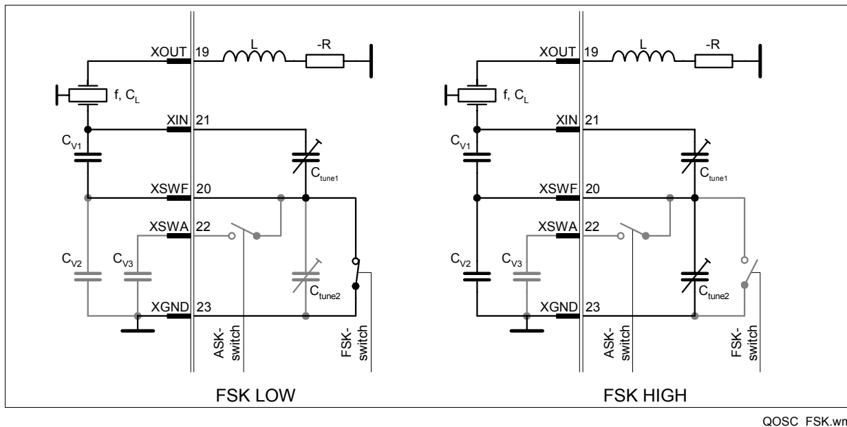
Figure 3-14 FSK modulation
