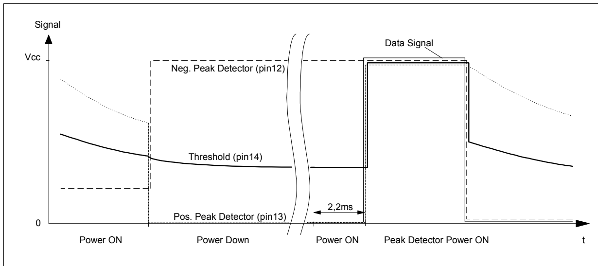
Figure 3-27 Power down mode
