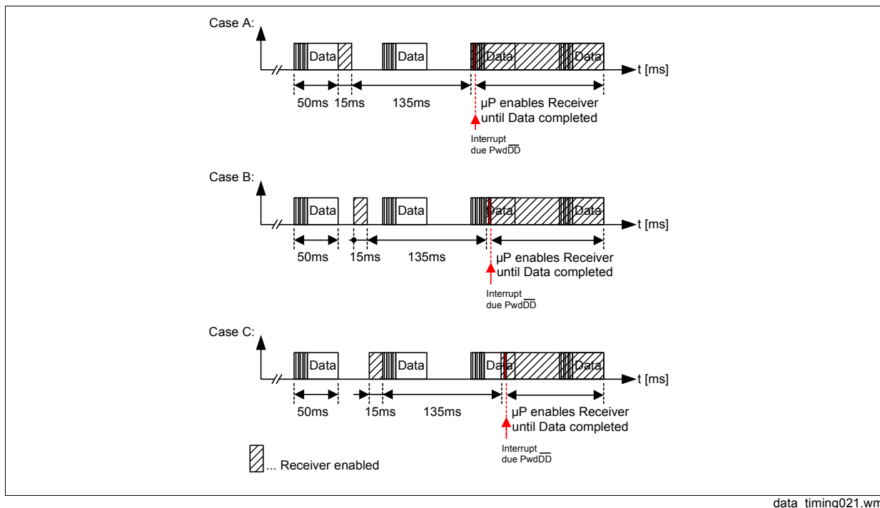
Figure 3-32 3 possible timings
