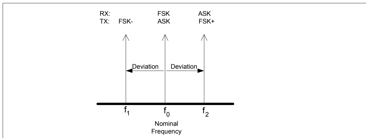
Figure 3-13 possible crystal oscillator frequencies
