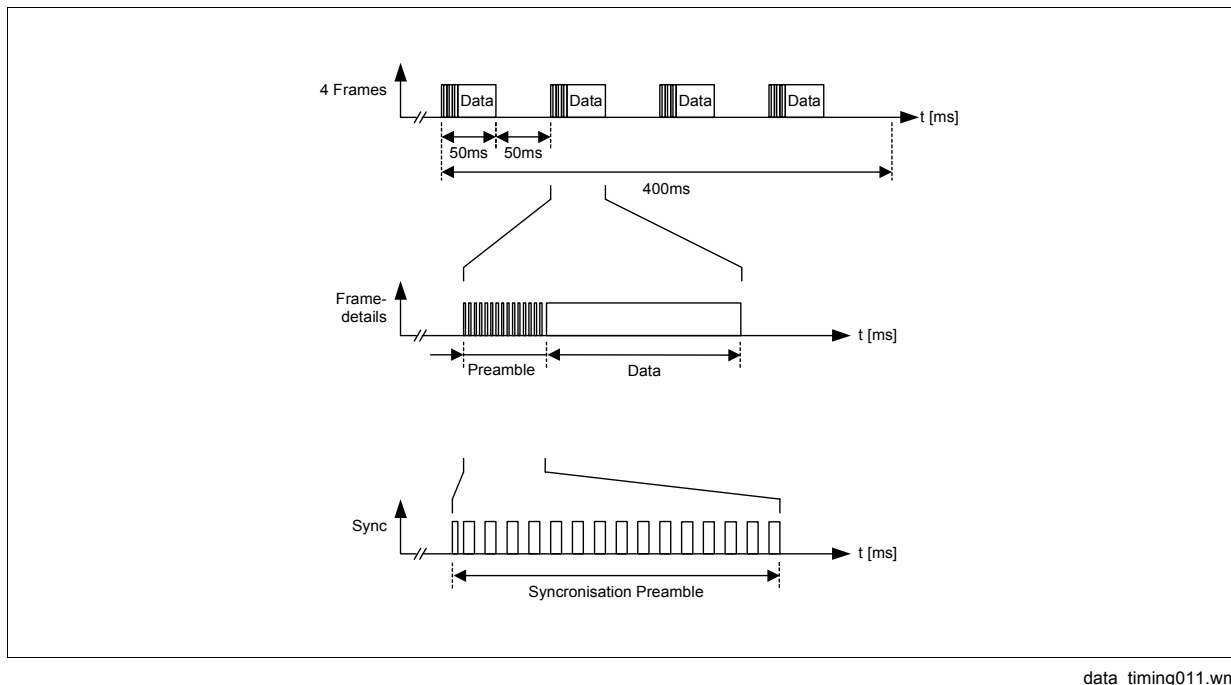
Figure 3-31 Example for transmitted Data-structure
