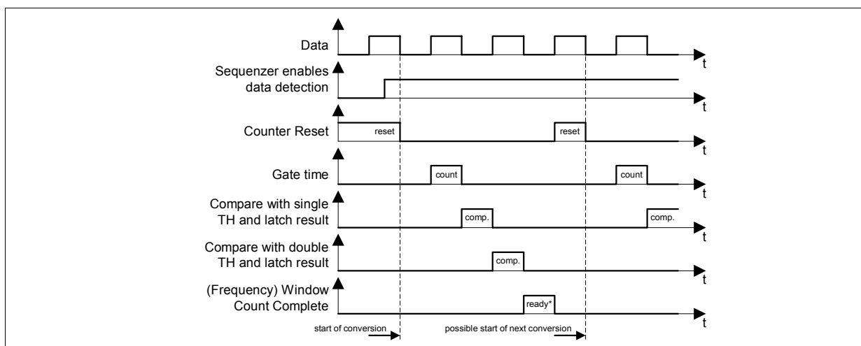
Figure 3-28 Frequency Detection timing in continuous mode
