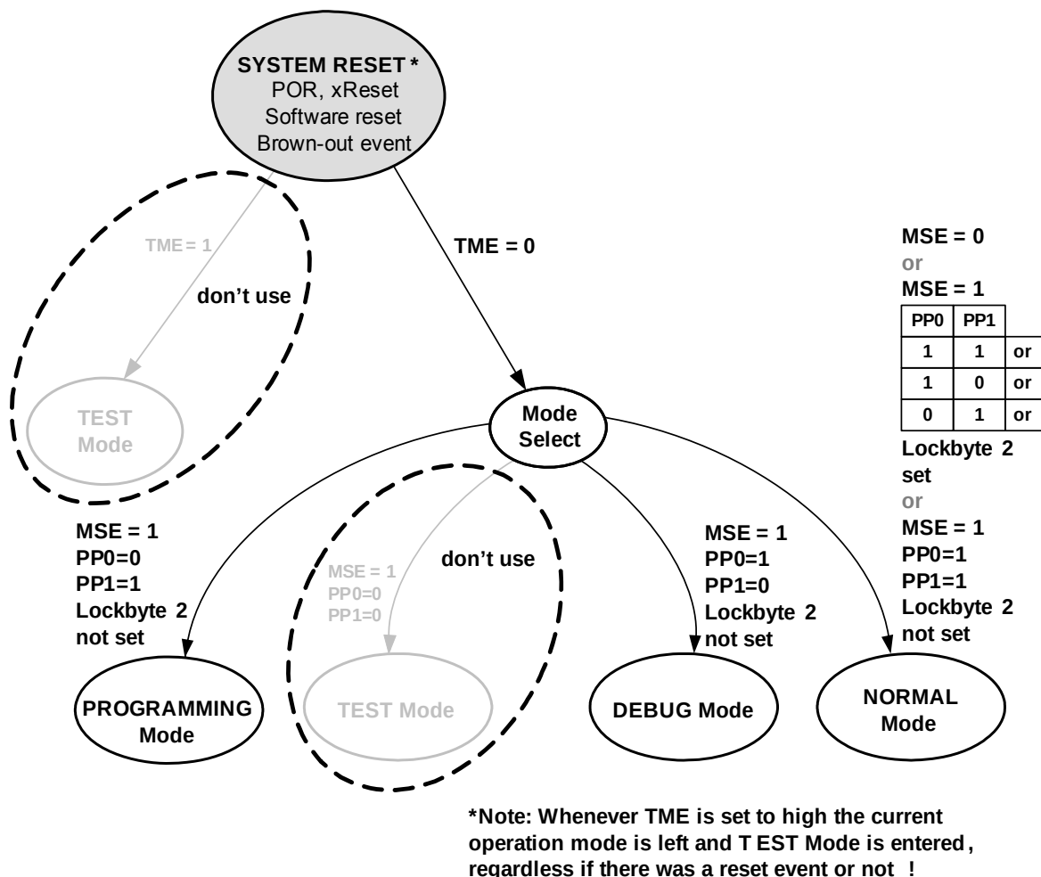
Figure 3 Operating Mode Selection of the PMA71xx after Reset
