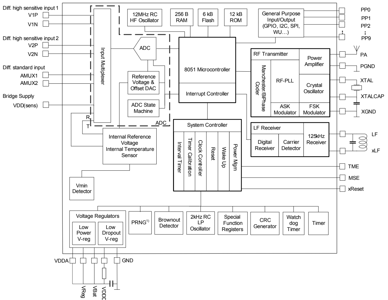
Figure 2 PMA71xx Block Diagram
