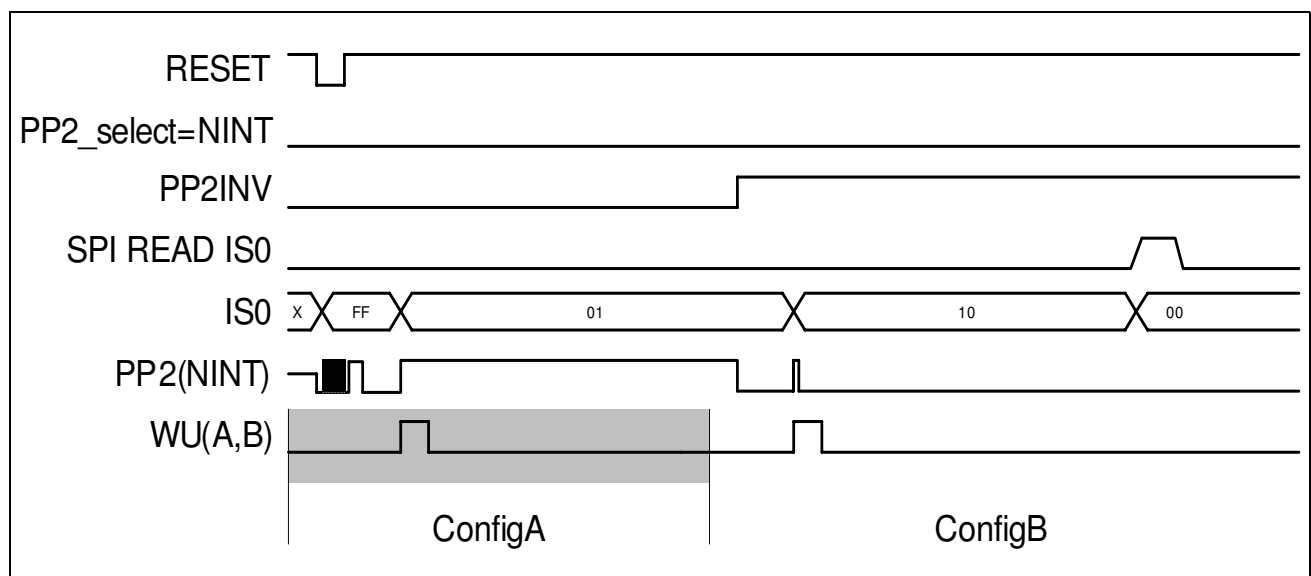
Figure 26 Interrupt Generation Waveform (Example for Configuration A+B)
