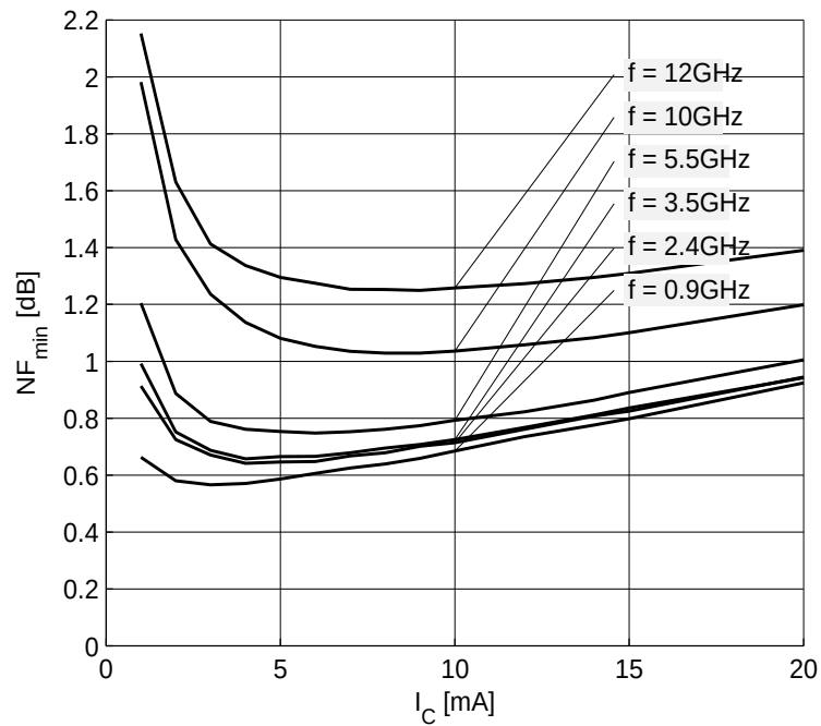
Figure 20 Noise Figure NF_{min} = f(I_C) , V_{CE} = 1.8\text{ V} , Z_S = Z_{opt} , f = \text{Parameter in GHz}
