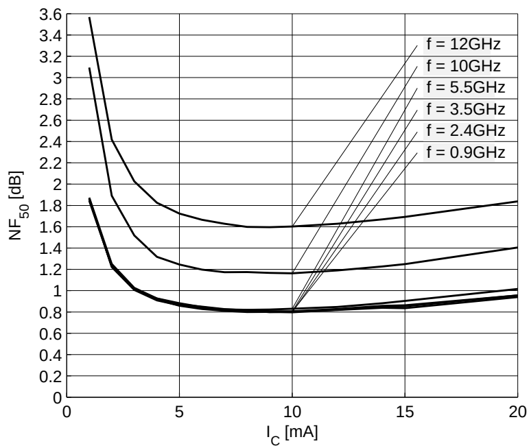
Figure 21 Noise Figure NF_{50} = f(I_C) , V_{CE} = 1.8\text{ V} , Z_S = 50\ \Omega , f = \text{Parameter in GHz}
