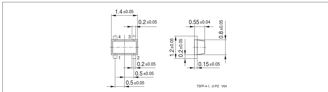
Figure 22 Package Outline
