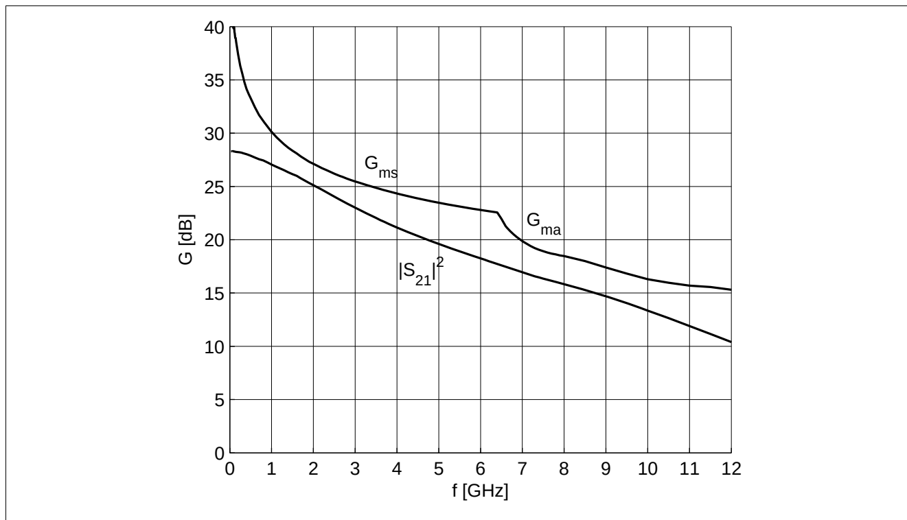
Figure 13 Gain G_{ma} , G_{ms} , |S_{21}|^2 = f(f) , V_{CE} = 1.8 V, I_C = 10 mA
