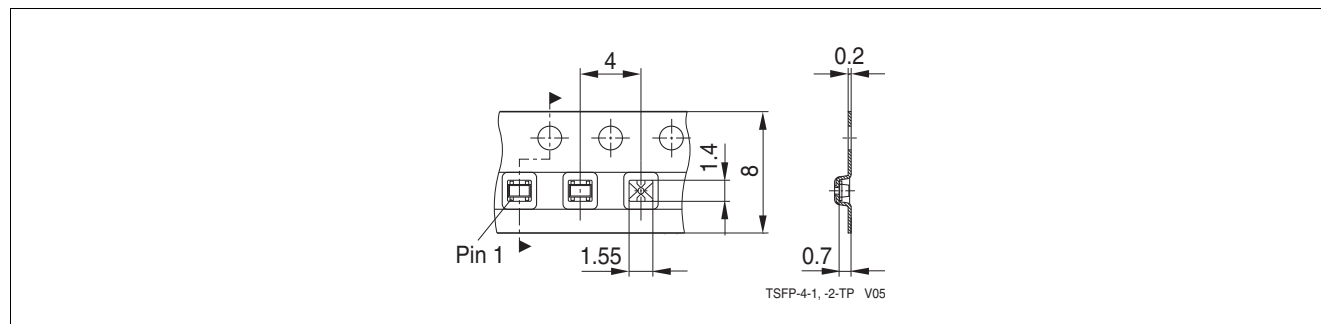
Figure 25 Tape Dimensions
