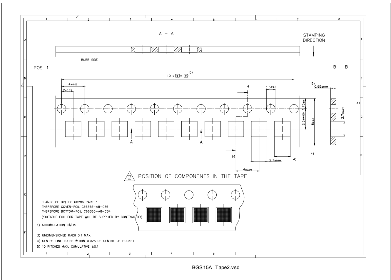
Figure 4 Tape Drawing for PG-TSNP-16-3
