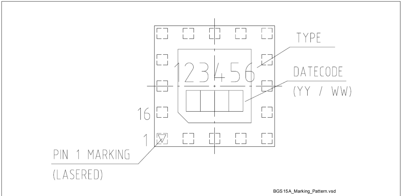
Figure 3 Pin Marking
