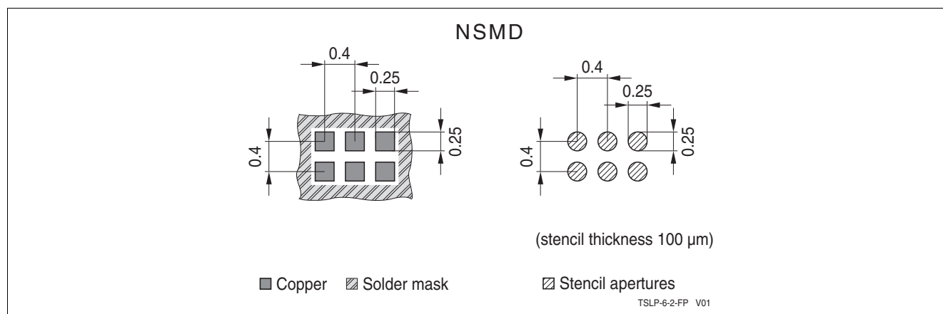
Figure 6 Footprint TSLP-6-2
