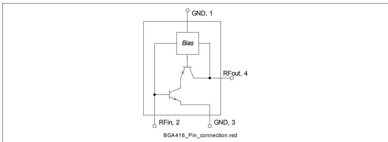
Figure 1 Pin connection
