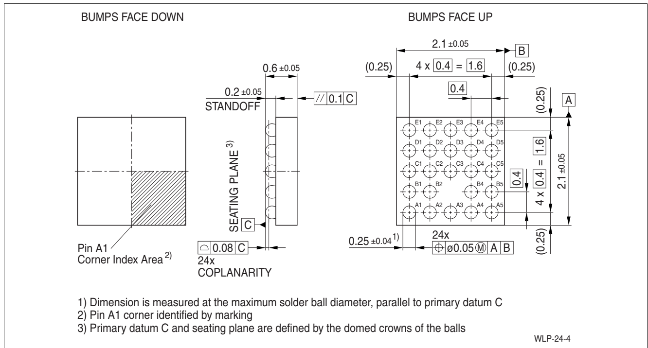
Figure 4 Package WLP-24-4
