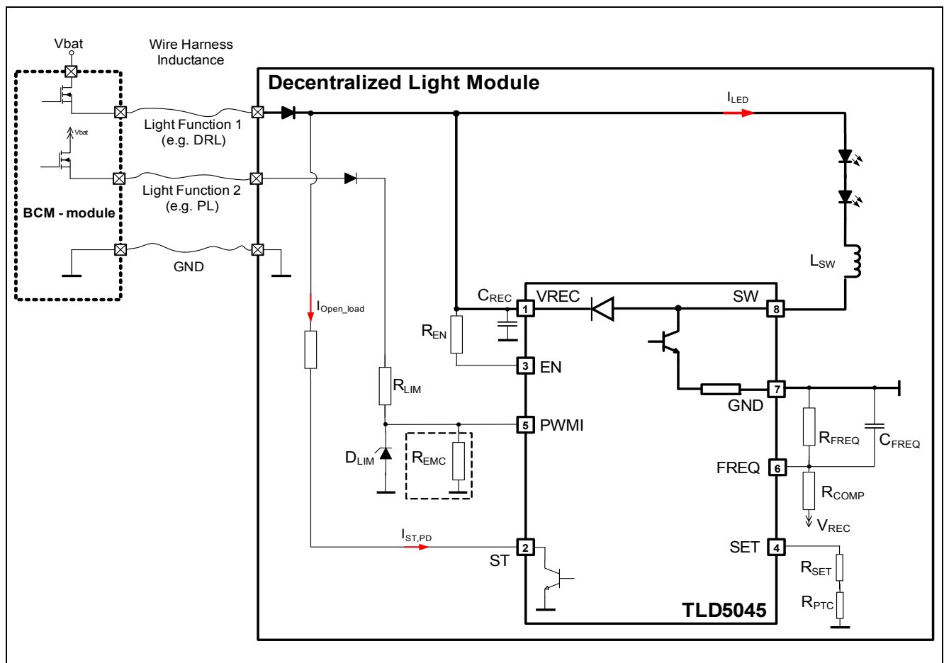
Figure 17 Application Diagram of Decentralized Light Module without \mu C (input config 3)
