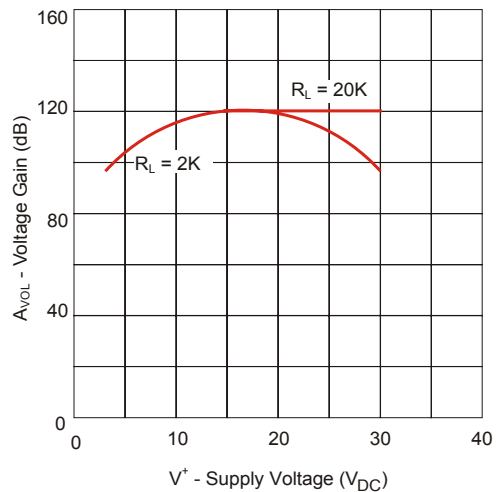
Figure 4. Voltage Gain
