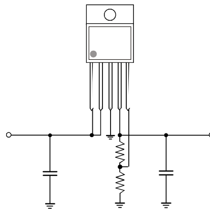
Adjustable Voltage Version
