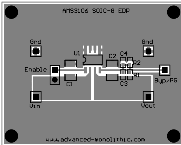
Figure 4: AMS3106 SOIC-8 Evaluation Board Top Side
