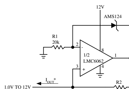
Precision 1 \mu A to 1mA Current Sources
