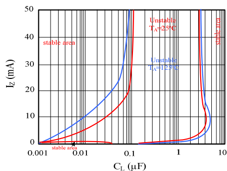
AMS431 Stability vs. Output Capacitor 25°C and 125°C
