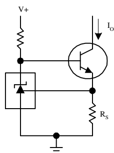
Constant Current Sink
