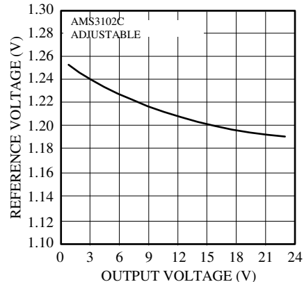
Reference Voltage
