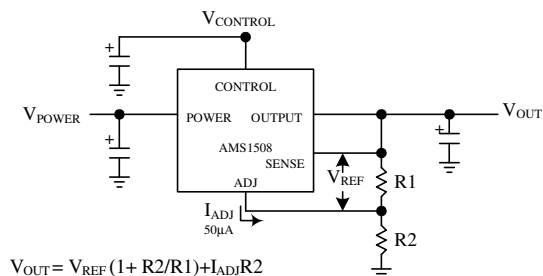
Figure 5. Setting Output Voltage
