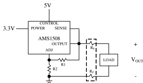
Figure 1. Conventional Load Sensing
