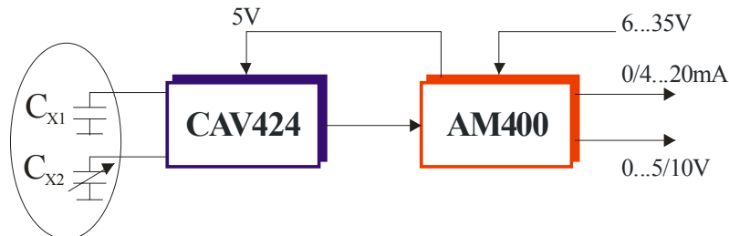
Figure 14: Application as a converter IC together with CAV424 for the measurement of capacitive V424 signals
