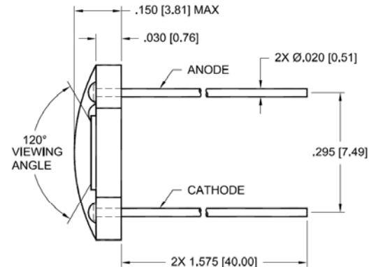
PACKAGE DIMENSIONS INCH [mm]
