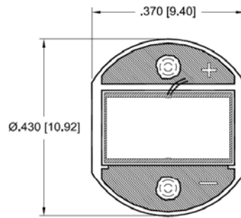
CHIP DIMENSIONS INCH [mm]
