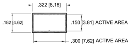
CHIP DIMENSIONS INCH [mm]
