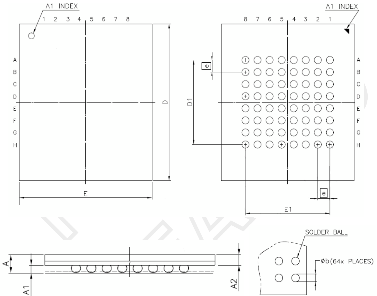
FIGURE 23. J1 64-ball Ball Grid Array, (11X13mm), Pitch 1mm package outline
