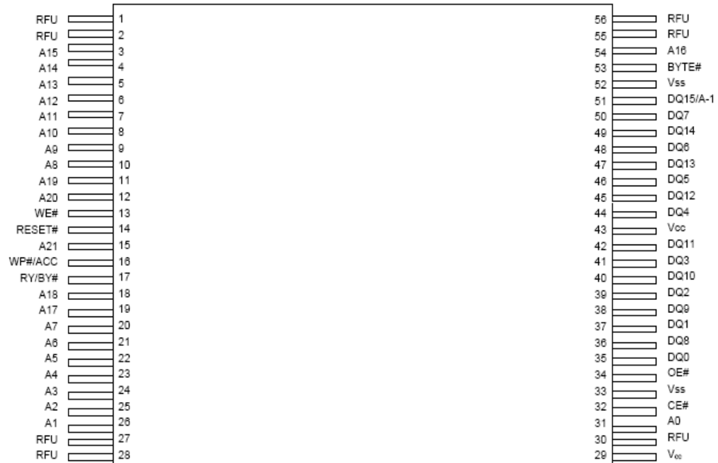
Figure 1. 56-pin Standard TSOP (Top View)
