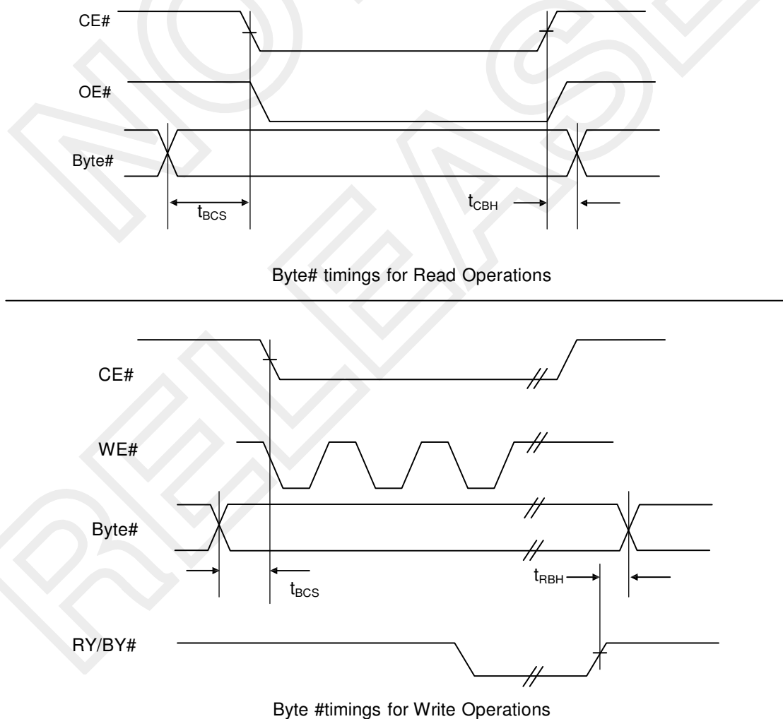
Figure 15. AC Waveforms for BYTE#
