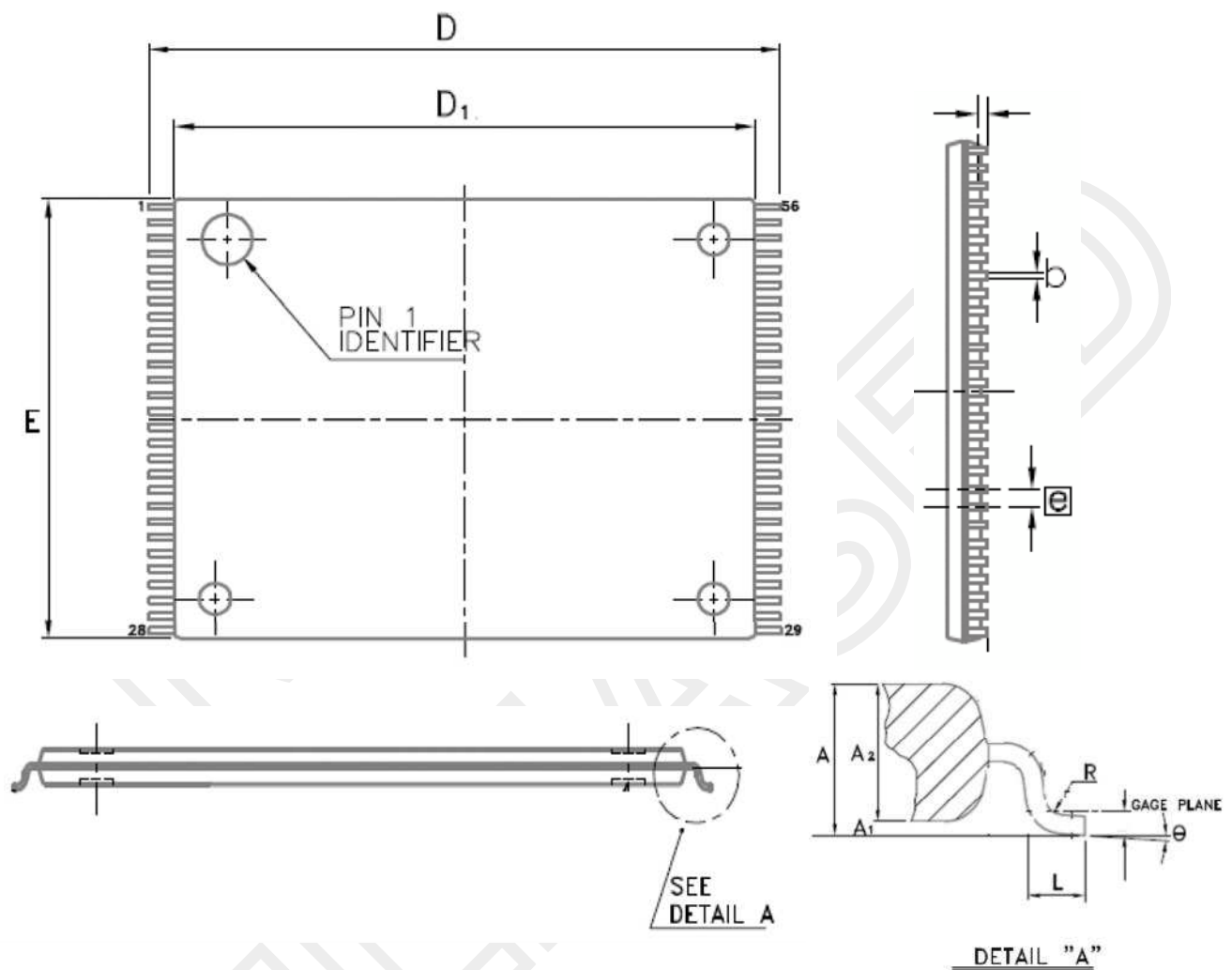
FIGURE 22. JT 56Pin TSOP (14x20mm) package outline
