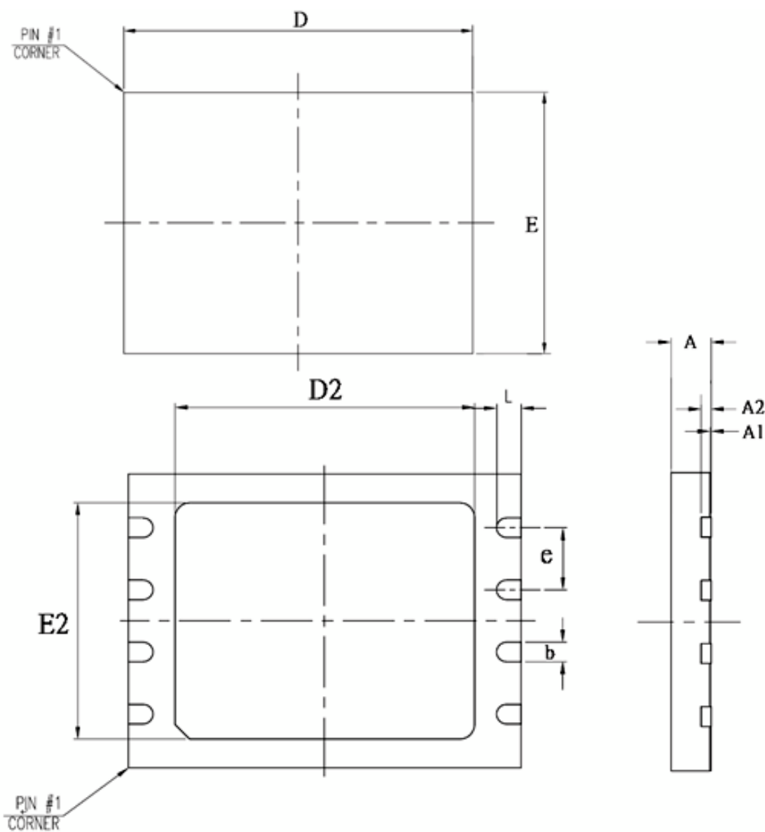
Figure 32. WSON (5x6mm)
