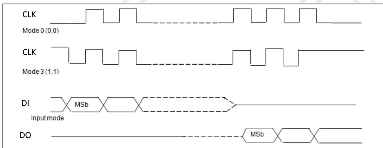
Figure 3. SPI Modes
