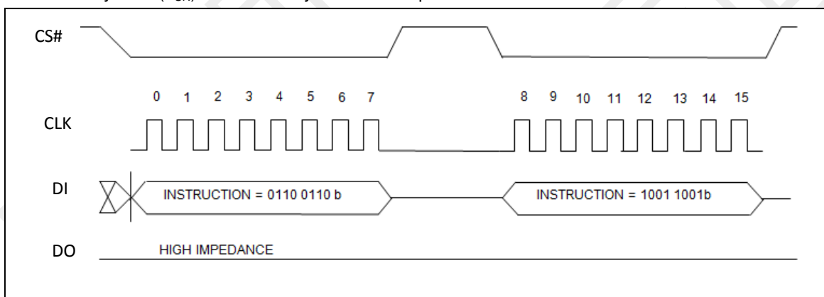
Figure 6. Reset-Enable and Reset Sequence Diagram
