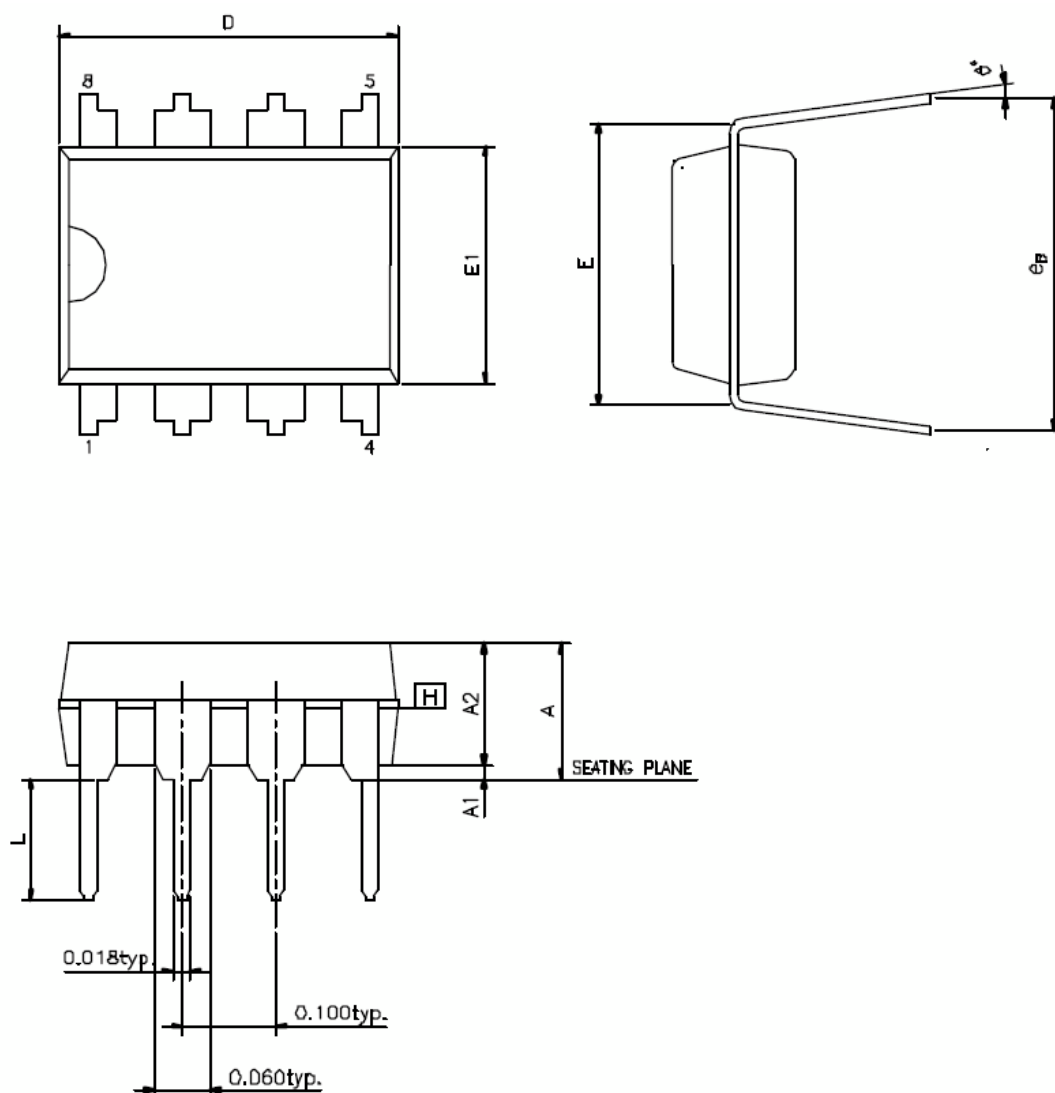
Figure 34. 8-pin SOIC
