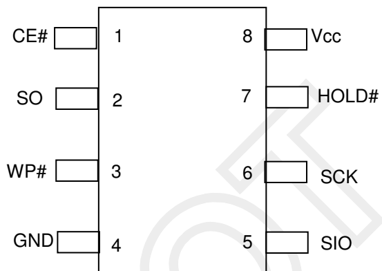
8-Pin SOIC
