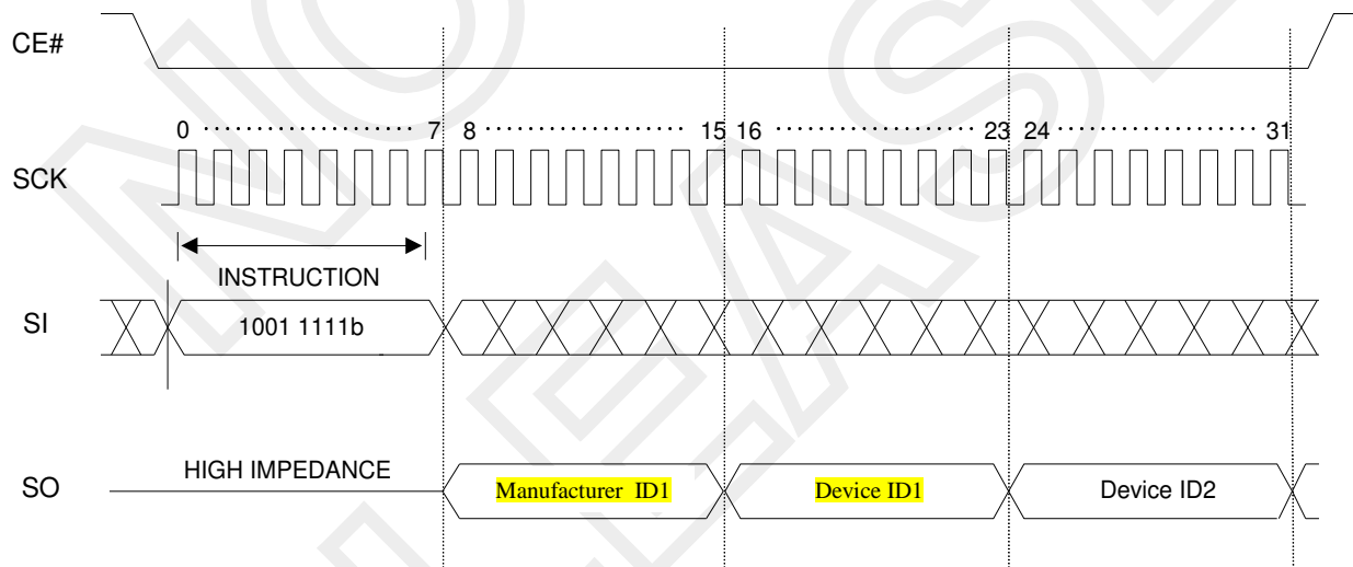
Figure 4. Read Product Identification by JEDEC ID READ Sequence
