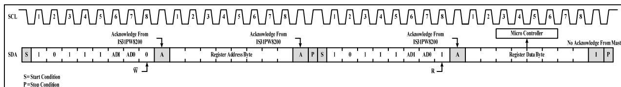
Figure 6 Reading from IS31PW8200
