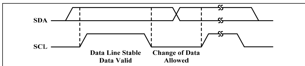
Figure 4 Bit Transfer
