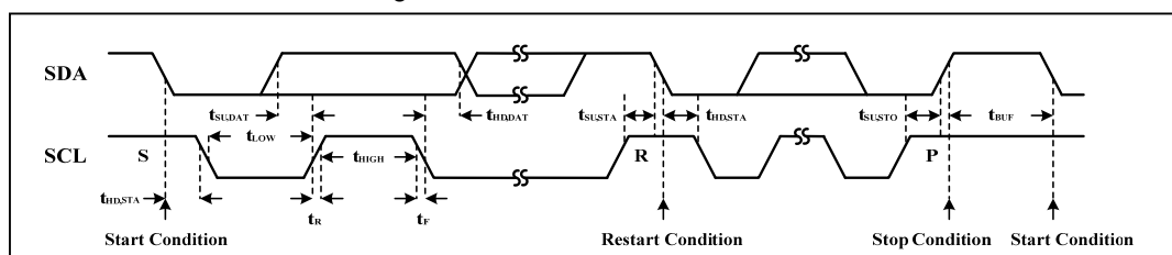
Figure 3 Interface Timing
