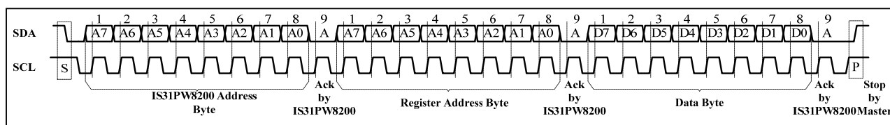
Figure 5 Writing to IS31PW8200
