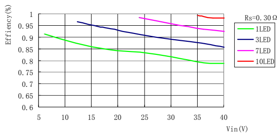
Efficiency vs. No. of LEDs L=47\mu\text{H} , R_s=0.30\Omega\text{hm}
