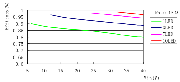
Efficiency vs. No. of LEDs L=47\mu\text{H} , R_s=0.15\Omega\text{hm}
