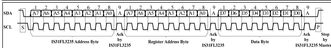
Figure 4 Writing to IS31FL3235(Typical)
