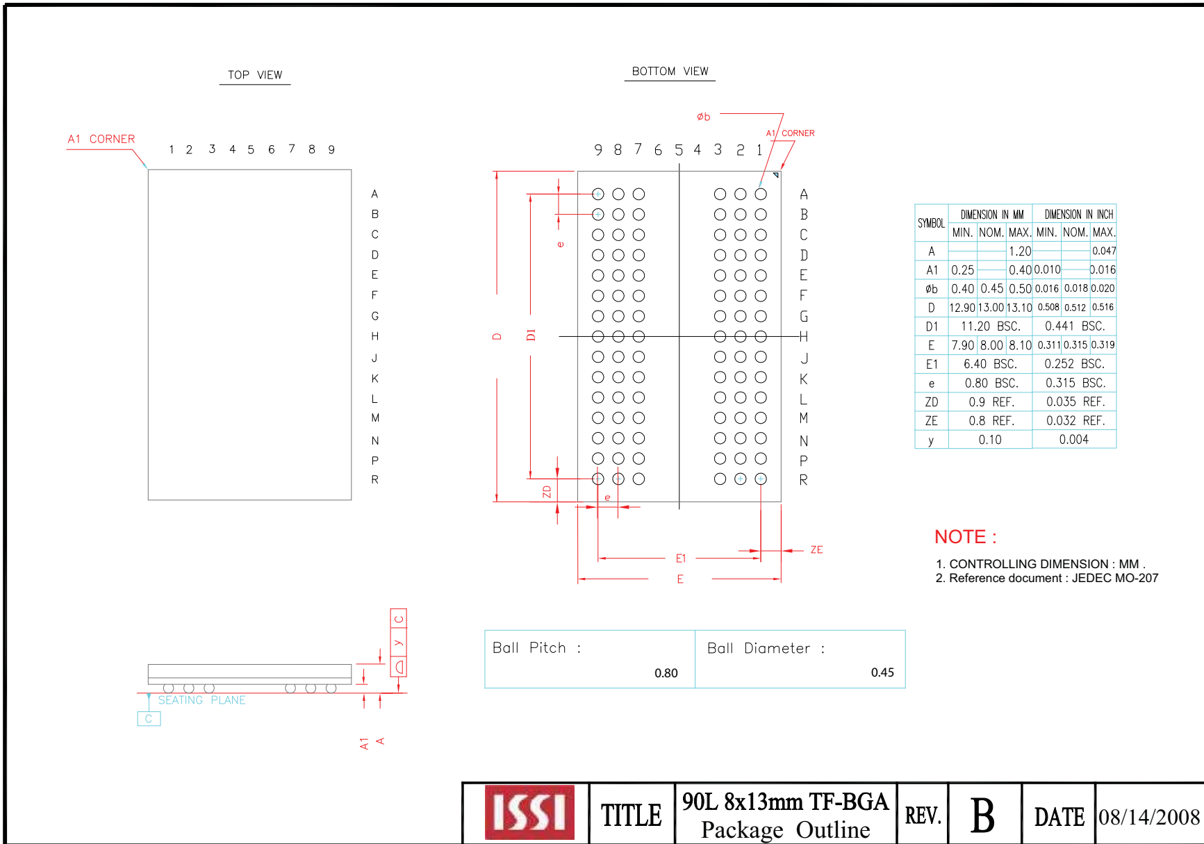
Figure9 : 90Ball FBGA Configuration
