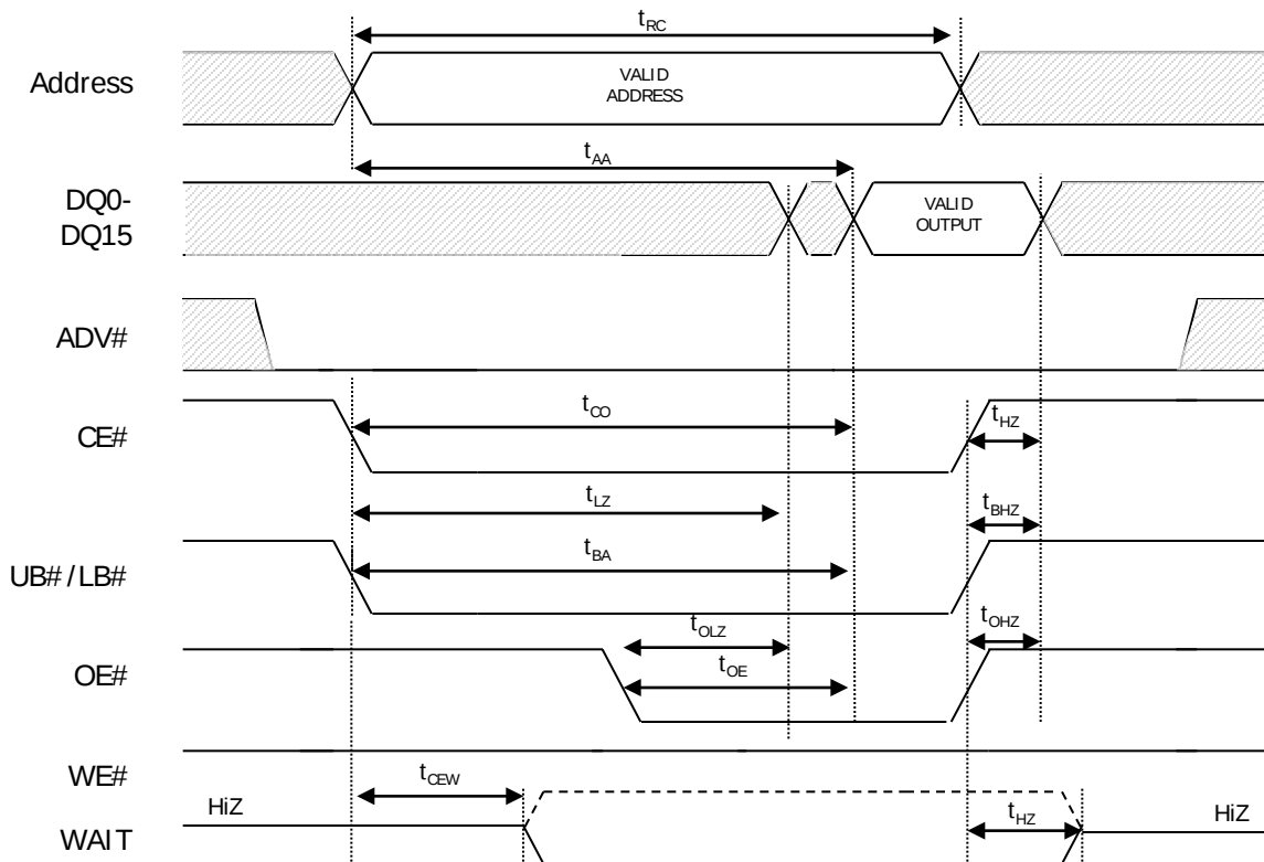
Figure 20: Asynchronous READ
