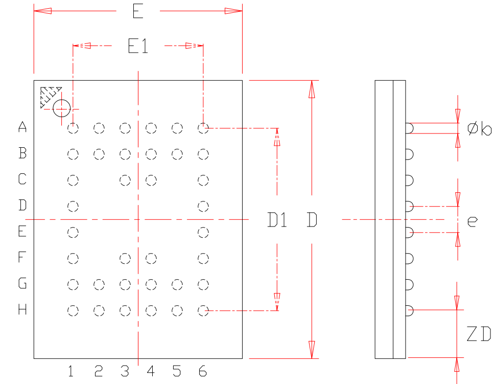
TOP VIEW
