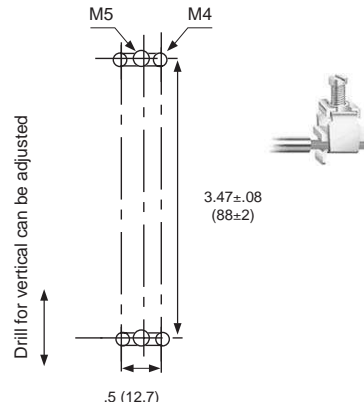
Figure 10 — DRS relay
