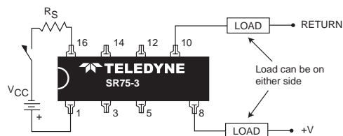
TYPICAL WIRING FOR DC APPLICATION
