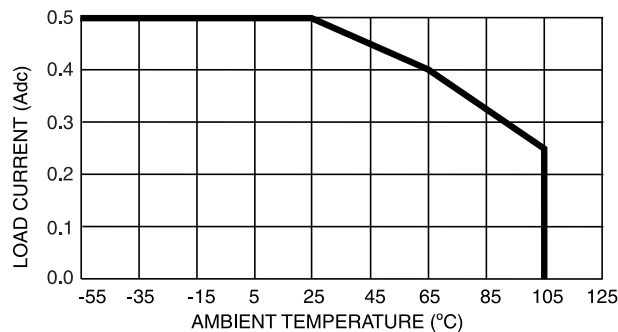
LOAD CURRENT DERATING CURVE FIGURE 4
