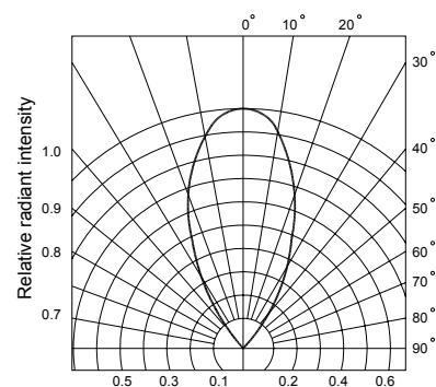
Fig.6 Radiation diagram
