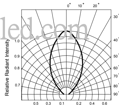
Fig.6 Radiant Diagram
