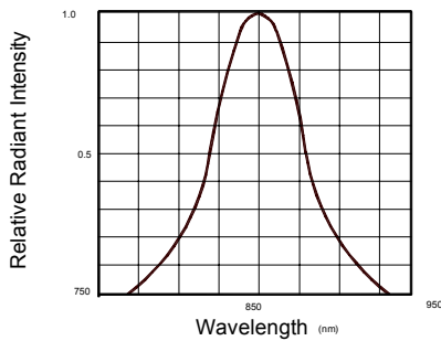
Fig.3 Spectral Distribution
