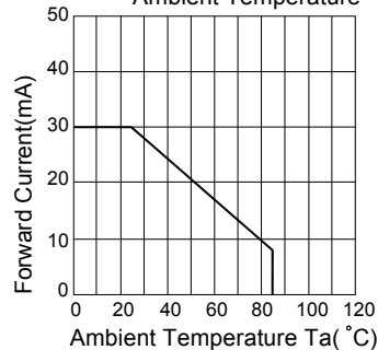
Fig.5 Forward Current Derating Curve VS. Ambient Temperature
