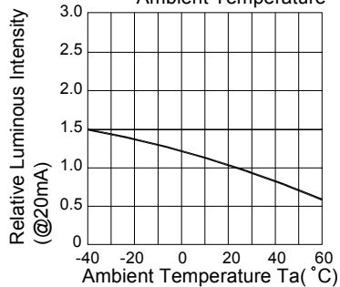
Fig.3 Relative Luminous Intensity VS. Ambient Temperature
